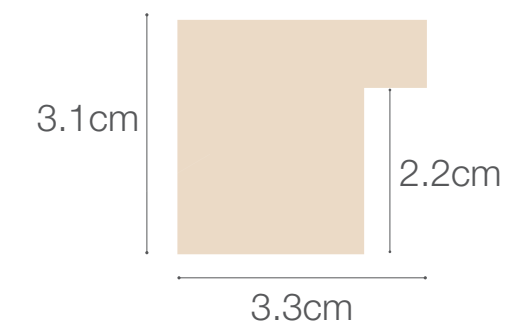
Profile: 6555-A#
