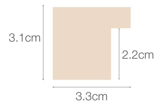
Profile: 6555-A#
